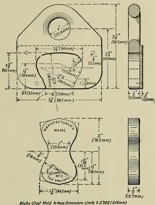
From A. S. T. M. Tent. Standards. Fig. 193.—Mould for Ascertaining the Tensile Strength of Bituminized Aggregates.
